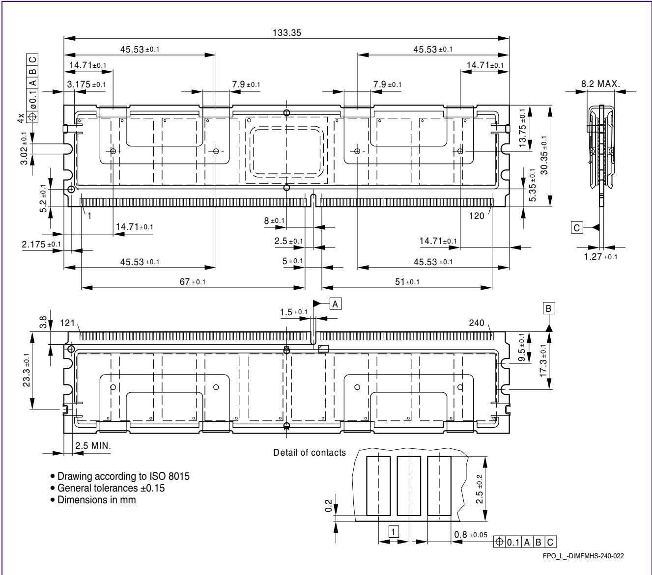
FIGURE 5 Package Outline L-DIM-240-22 with Full Module Heat Sink
