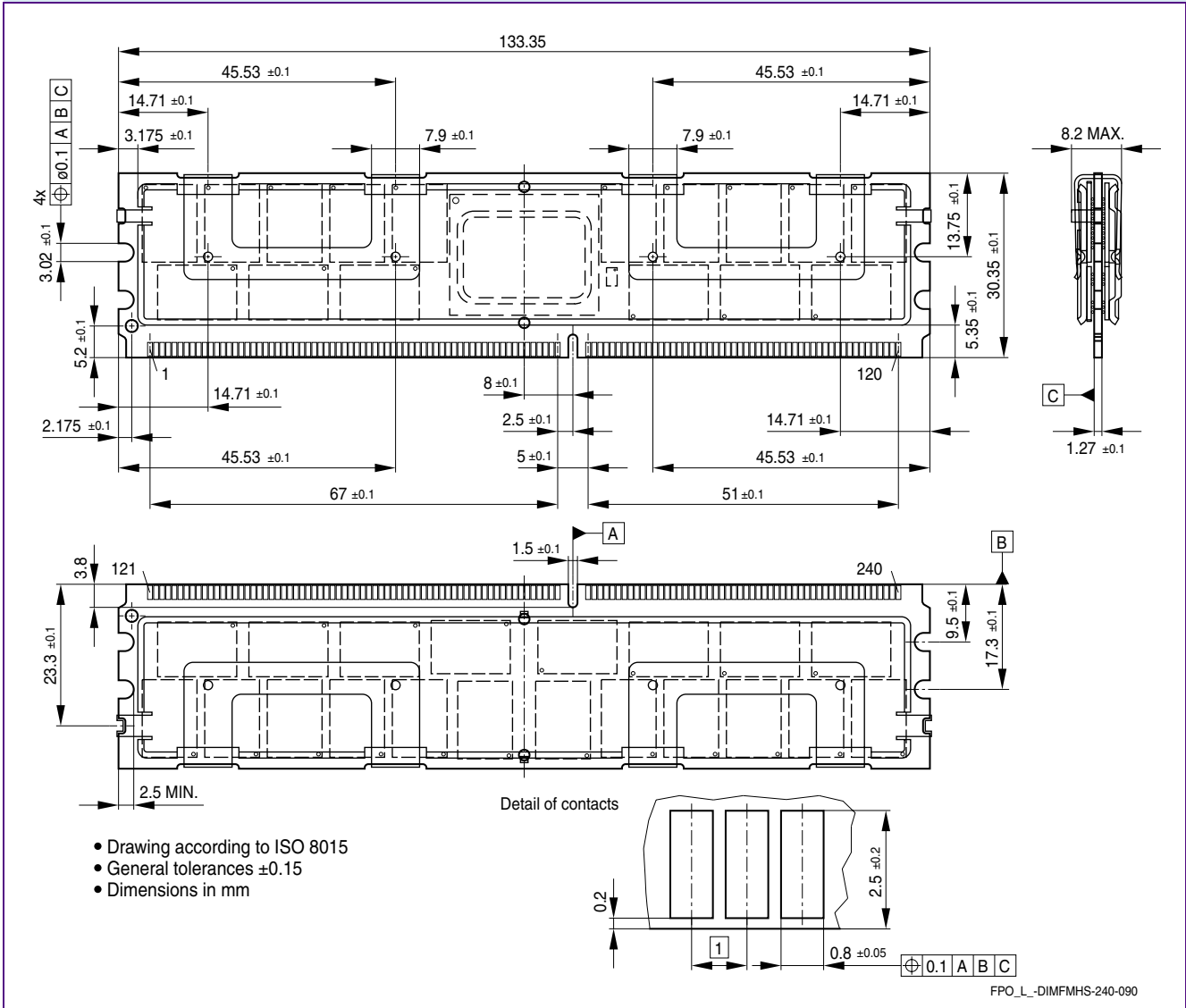
Package Outline L-DIM-240-90 Full Module Heat Sink
