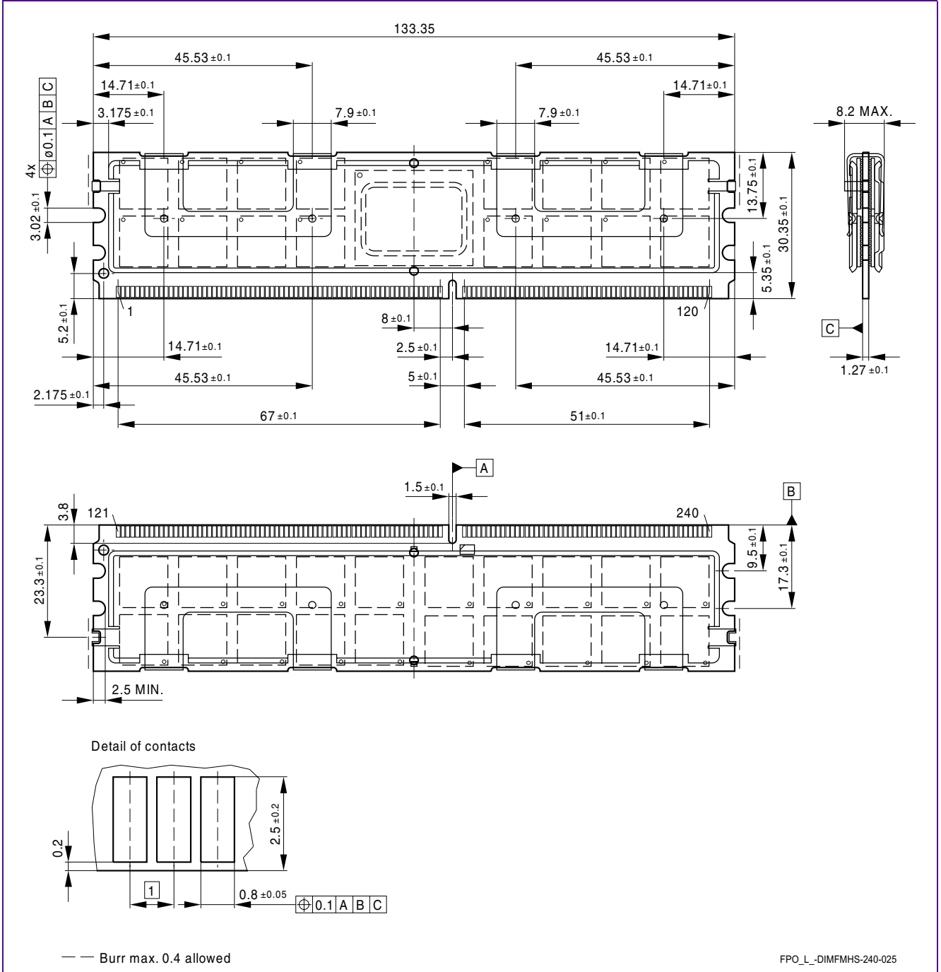
FIGURE 6 Package Outline L-DIM-240-25 with Full Module Heat Sink
