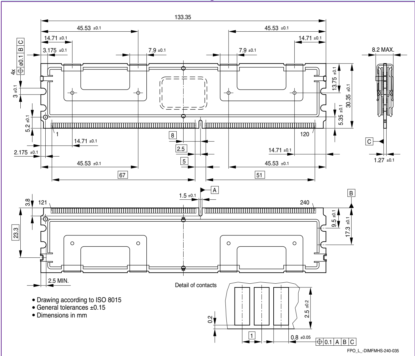
Package Outline L-DIM-240-35 with Full Module Heat Sink
