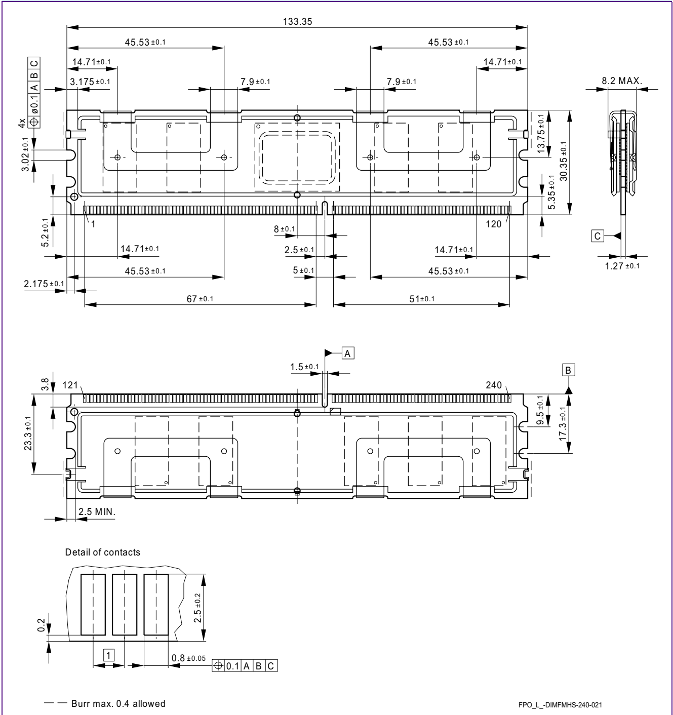
FIGURE 4 Package Outline L-DIM-240-21 with Full Module Heat Sink
