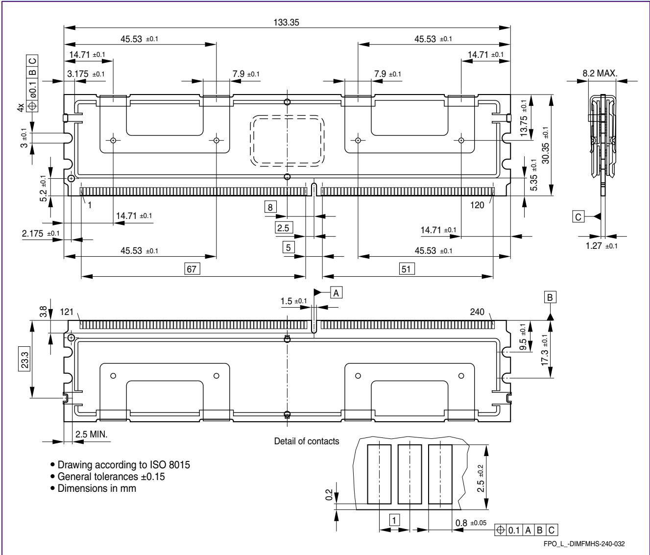
Package Outline L-DIM-240-32 with Full Module Heat Sink
